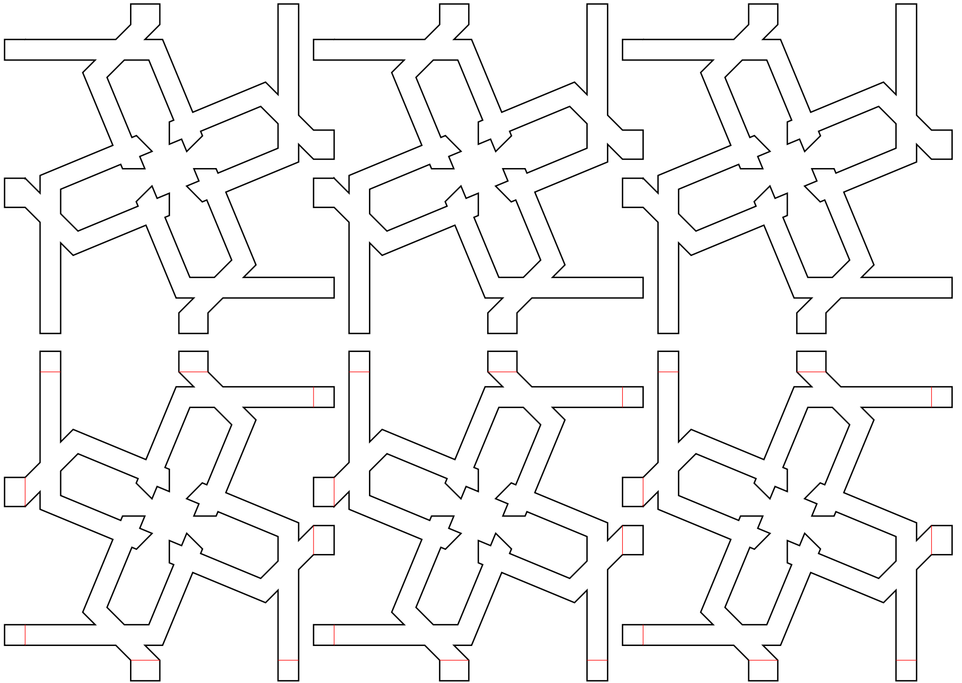
Black lines: cut; red lines: score. Cut two copies of this page for a two-layer cube. Craig S. Kaplan, 2017
